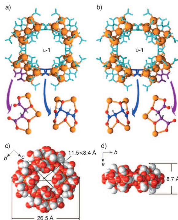
Figure 1. Ball-and-stick representations of a) L-1 b) D-1 (upper views; Fe orange spheres, C cyan, hydrogen atoms omitted for clarity) and two coordination modes for L-(–)-tartarate in L-1 and for D-(+)-tartarate in D-1 (lower views; O red, H gray). c), d) Space-filling representations of the {Fe 28 } wheel. Fe orange, O red, C gray, hydrogen atoms omitted for clarity.
